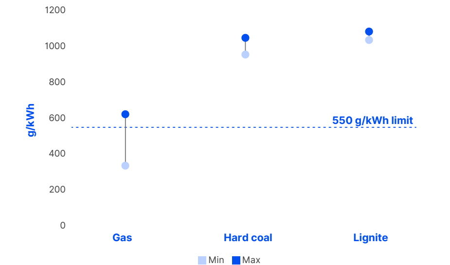
Figure 16: Ranges of the carbon dioxide emission of gas, hard coal and lignite-fired power plants per generated volume
