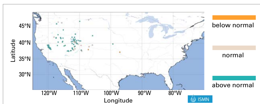
Figure 10. Soil moisture status down to 0.51 m depth in September 2023 in the contiguous United States. The reference data are the monthly averaged soil moisture of all Septembers 2008–2015. Due to limited data availability, data from only 88 stations located in the United States could be analysed.
