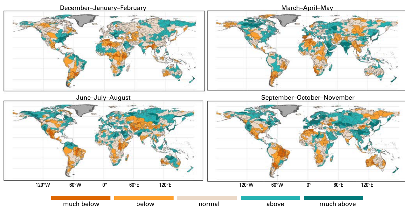
Figure 12. Seasonal actual evapotranspiration (AET) in 2023 as ranked with respect to the historical period 1991–2020 based on an ensemble of five GHMSs
