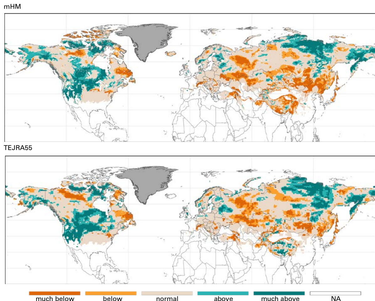
Figure A10. March 2023 snow water equivalent anomaly compared to the reference period (1991–2020)
